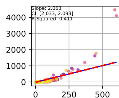
(Stochastic Binarization)
